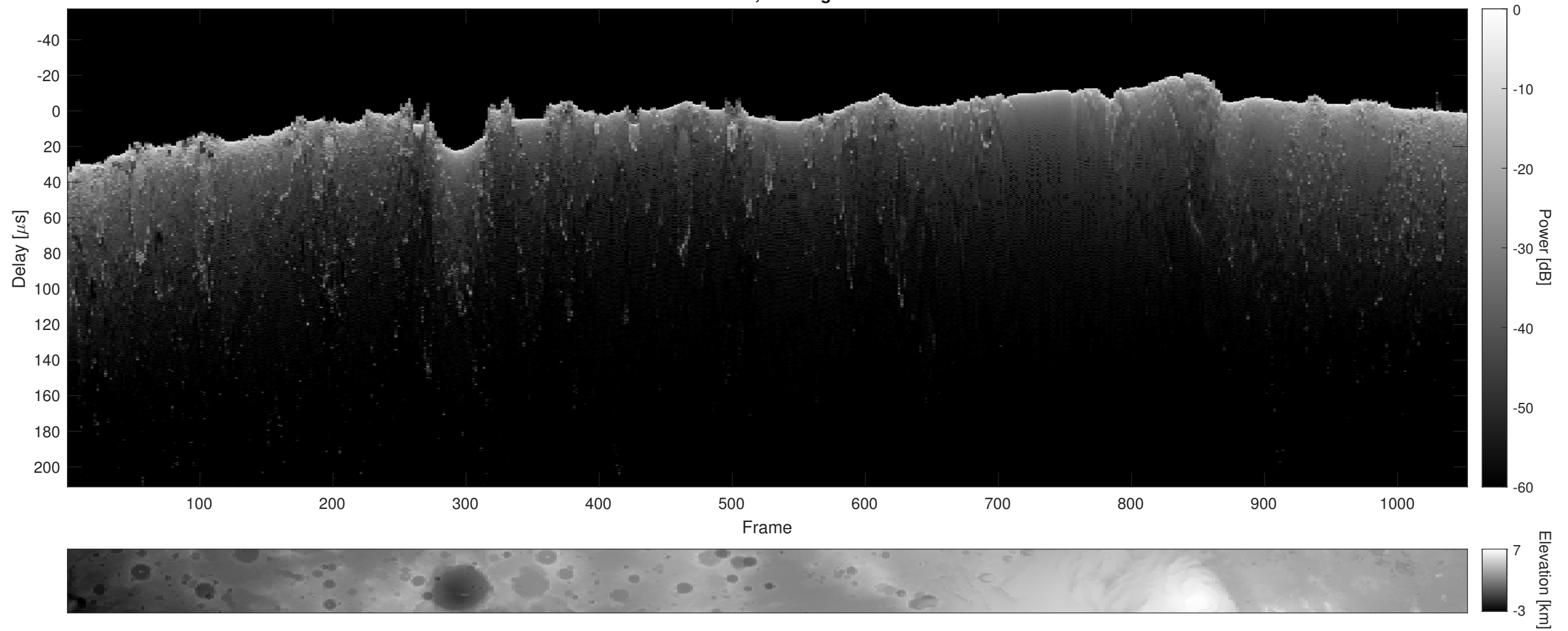
Orbit 2727, Cluttergram
