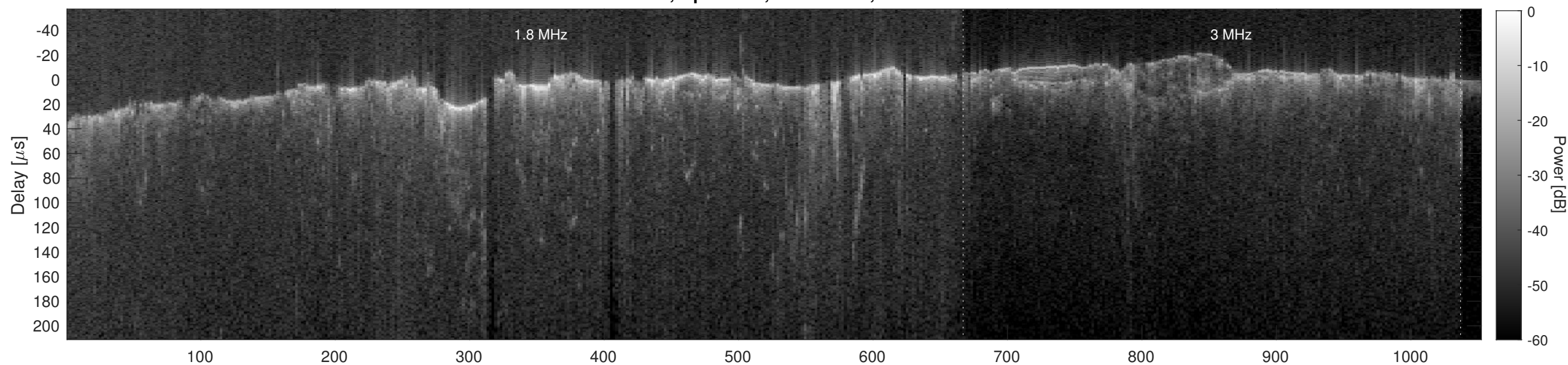
Orbit 2727, Cluttergram
