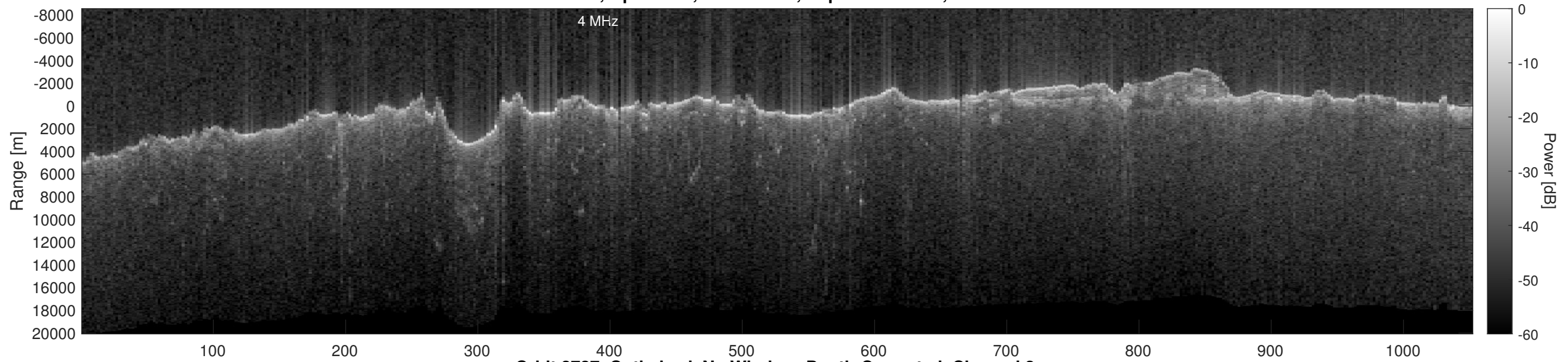
Orbit 2727, Optimized, No Window, Depth-Corrected, Channel 2
