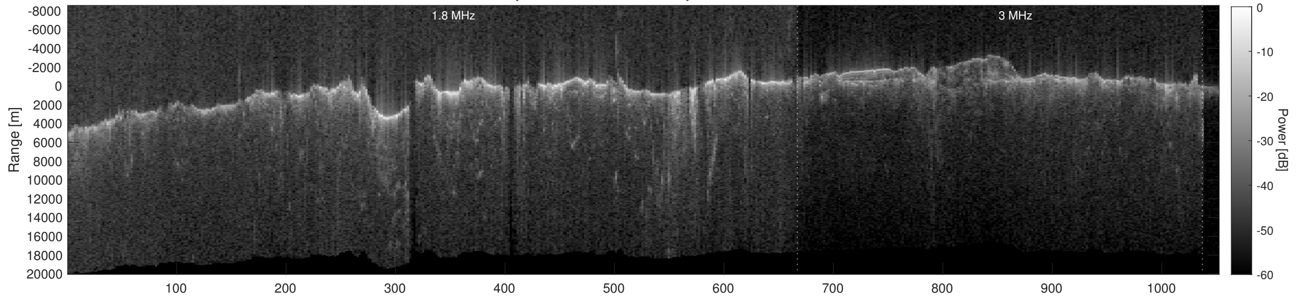
Orbit 2727, Depth-Corrected Cluttergram
