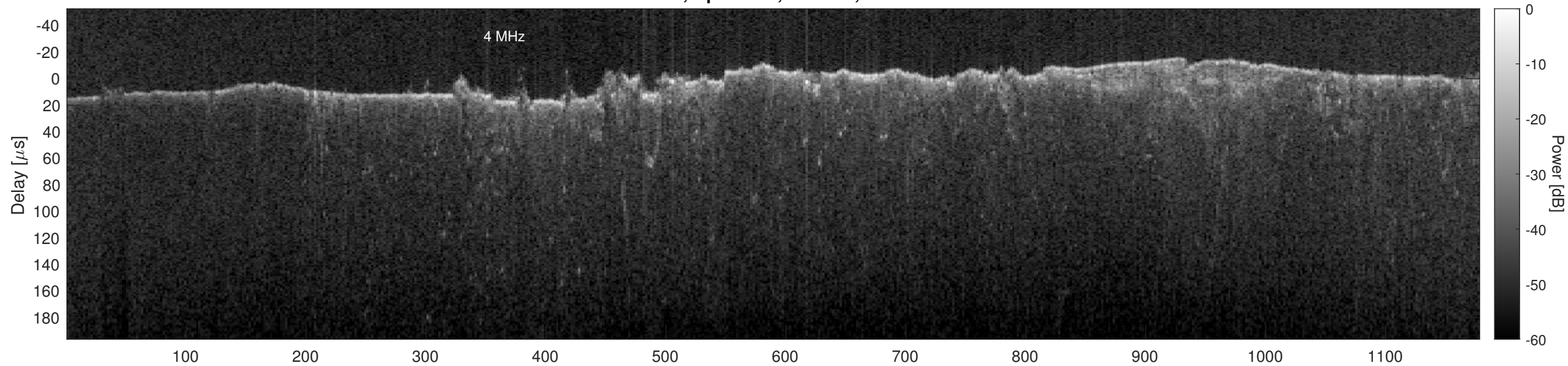
Orbit 2728, Optimized, Window, Channel 2
