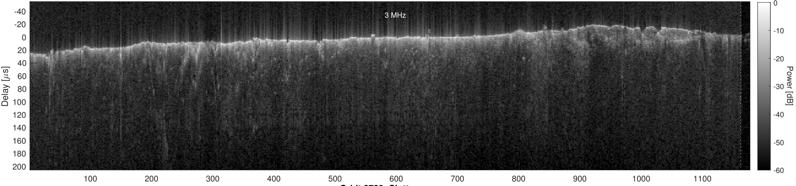
Orbit 2729, Cluttergram
