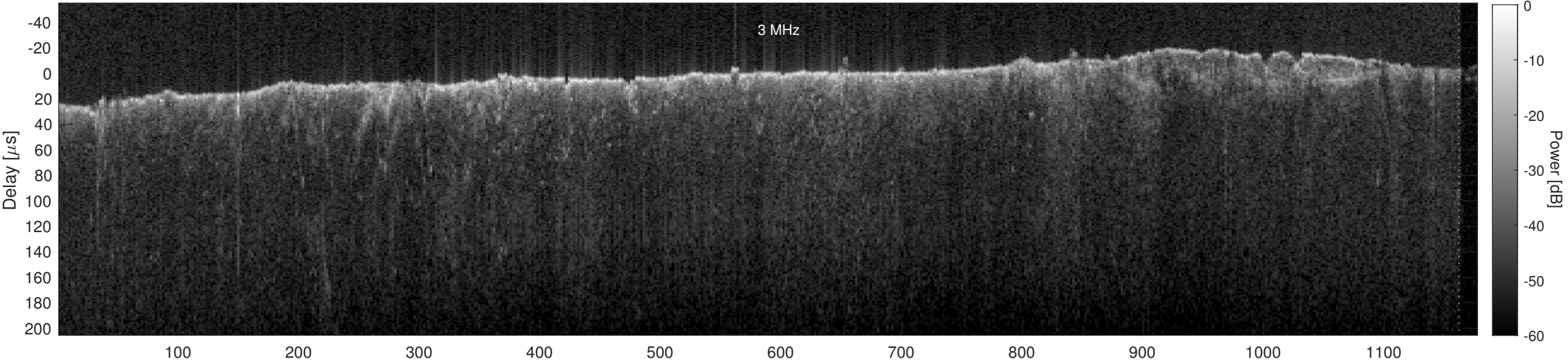
Orbit 2729, Cluttergram
