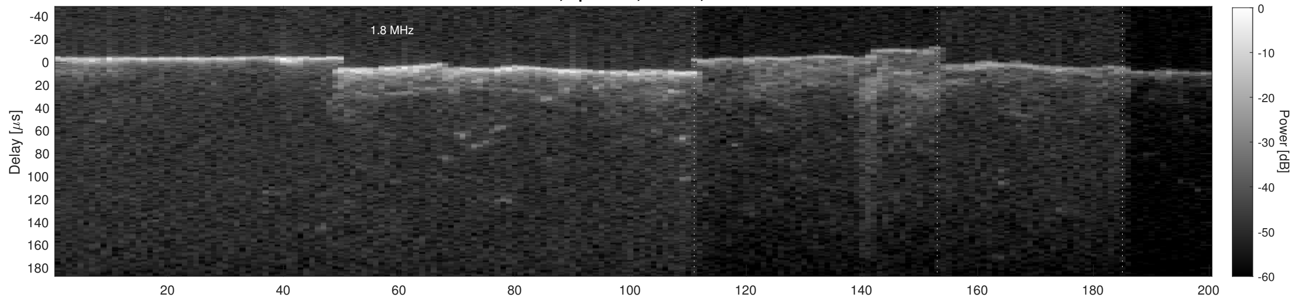
Orbit 2730, Cluttergram
