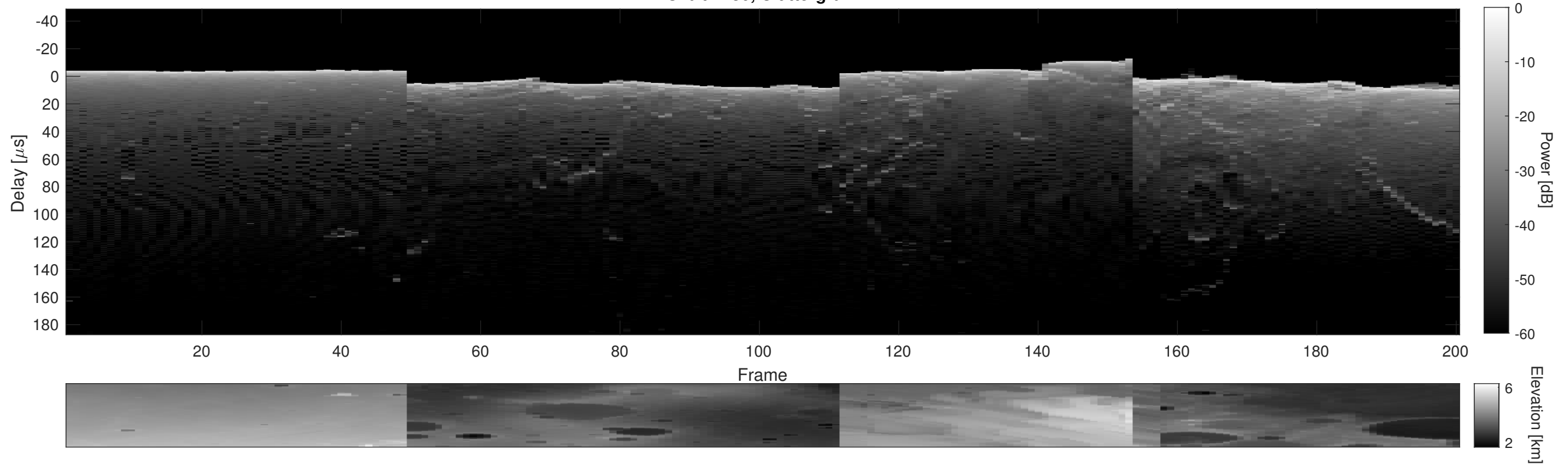
Orbit 2730, Cluttergram
