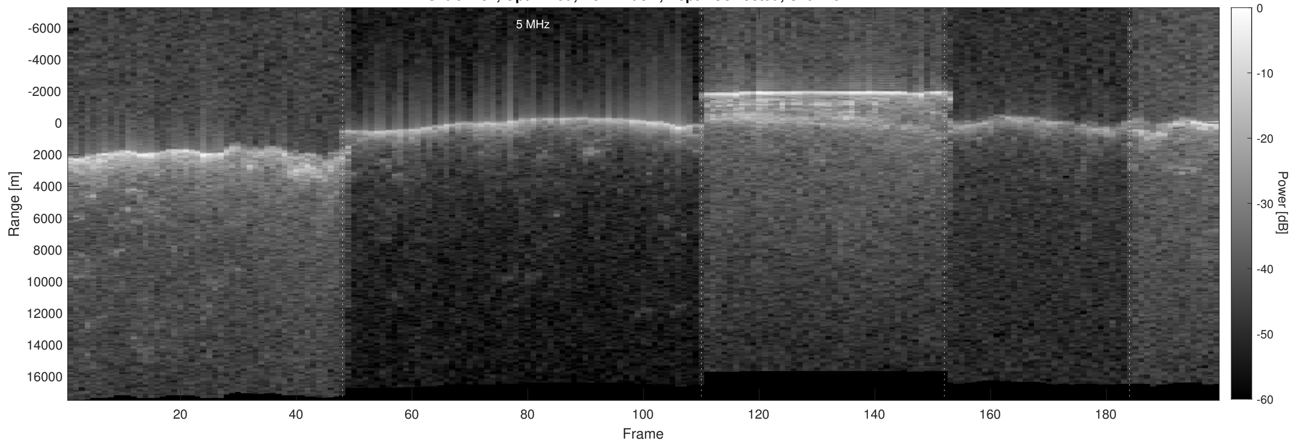
Orbit 2731, Optimized, No Window, Depth-Corrected, Channel 2
