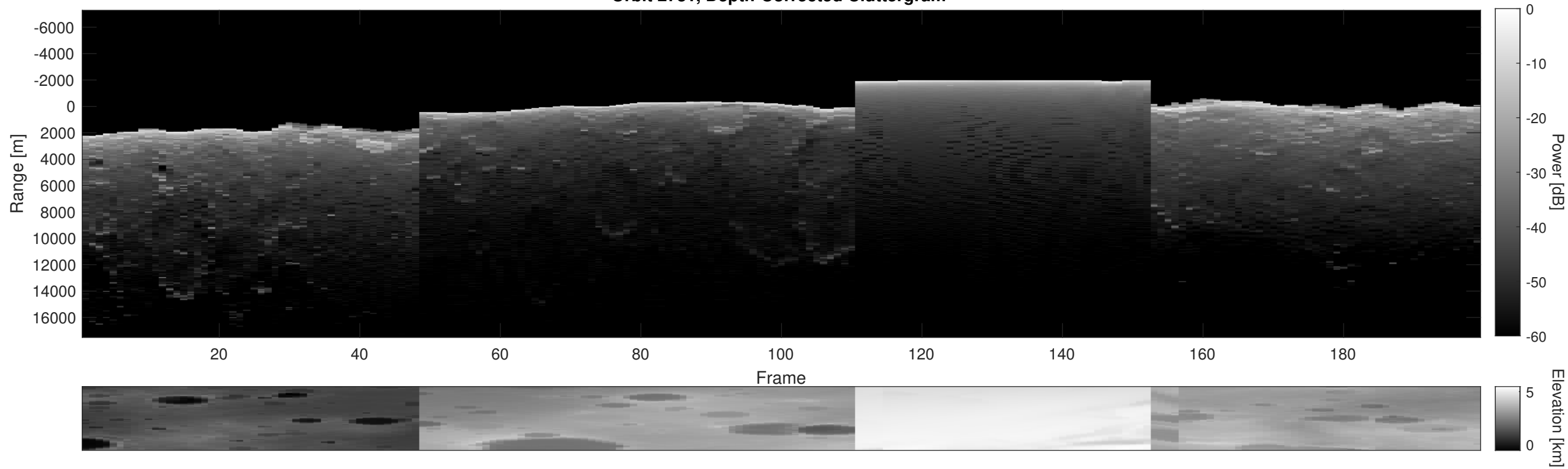
Orbit 2731, Depth-Corrected Cluttergram
