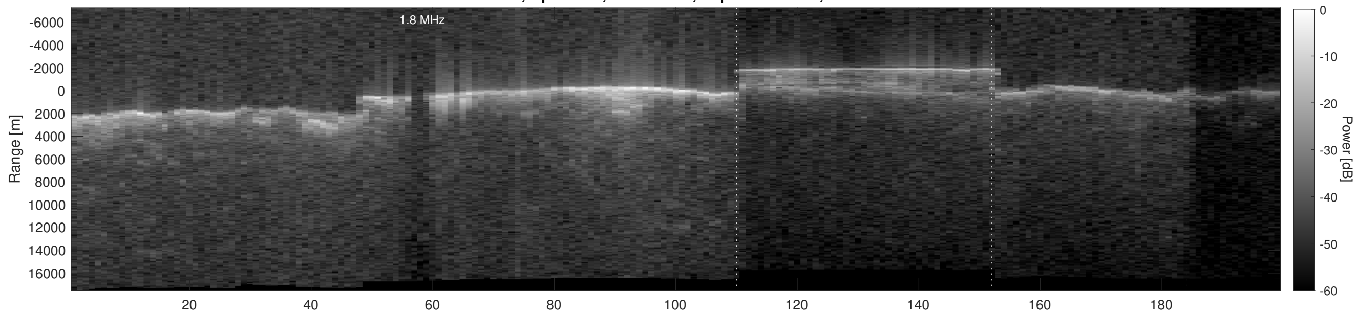
Orbit 2731, Depth-Corrected Cluttergram
