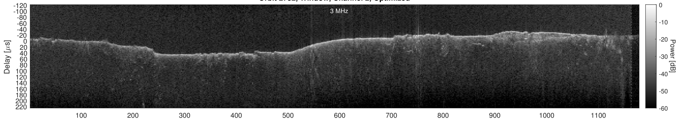
Orbit 2732, Cluttergram
