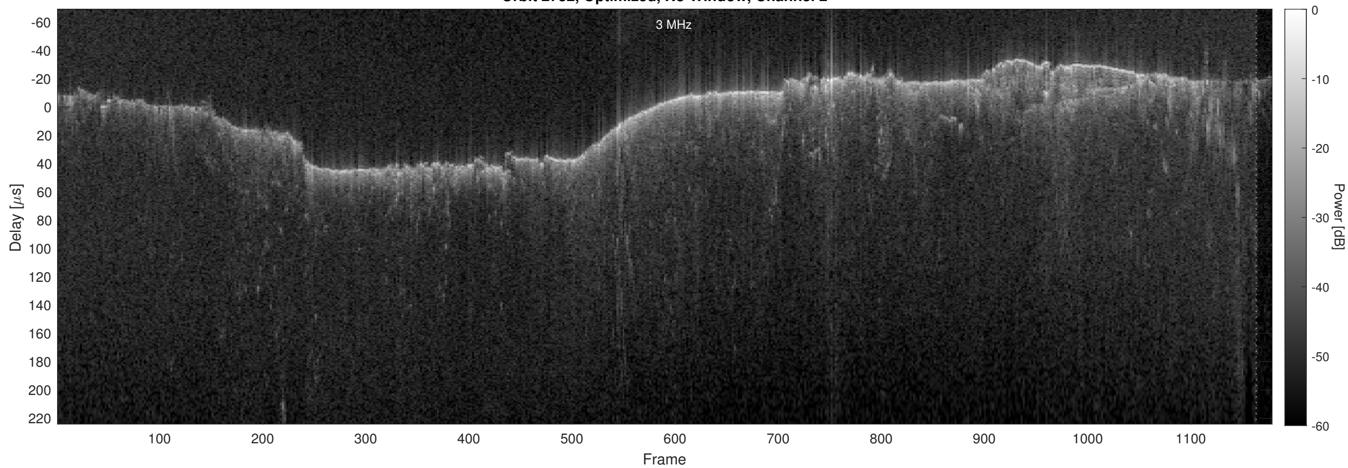
Orbit 2732, Optimized, No Window, Channel 2
