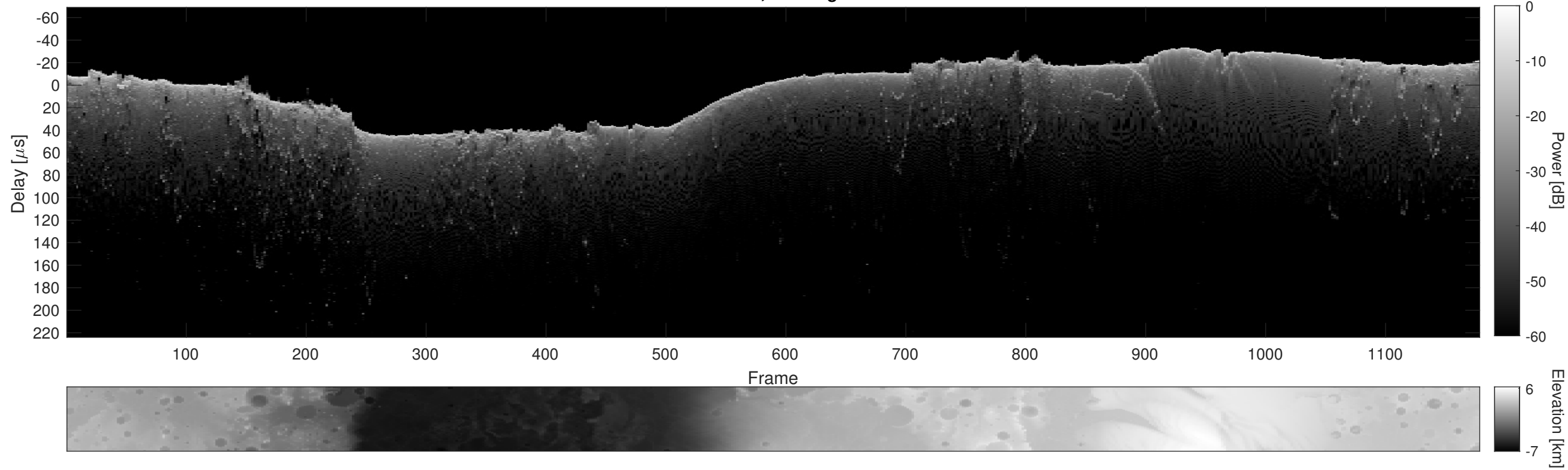
Orbit 2732, Cluttergram
