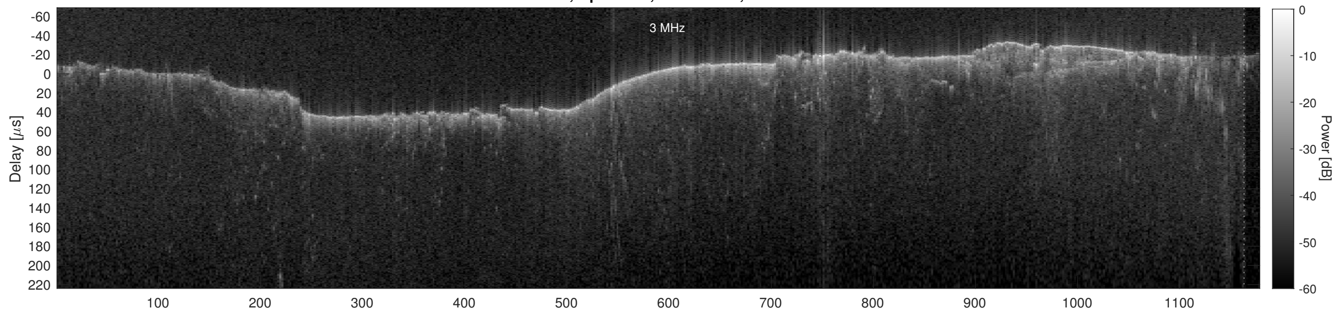
Orbit 2732, Cluttergram
