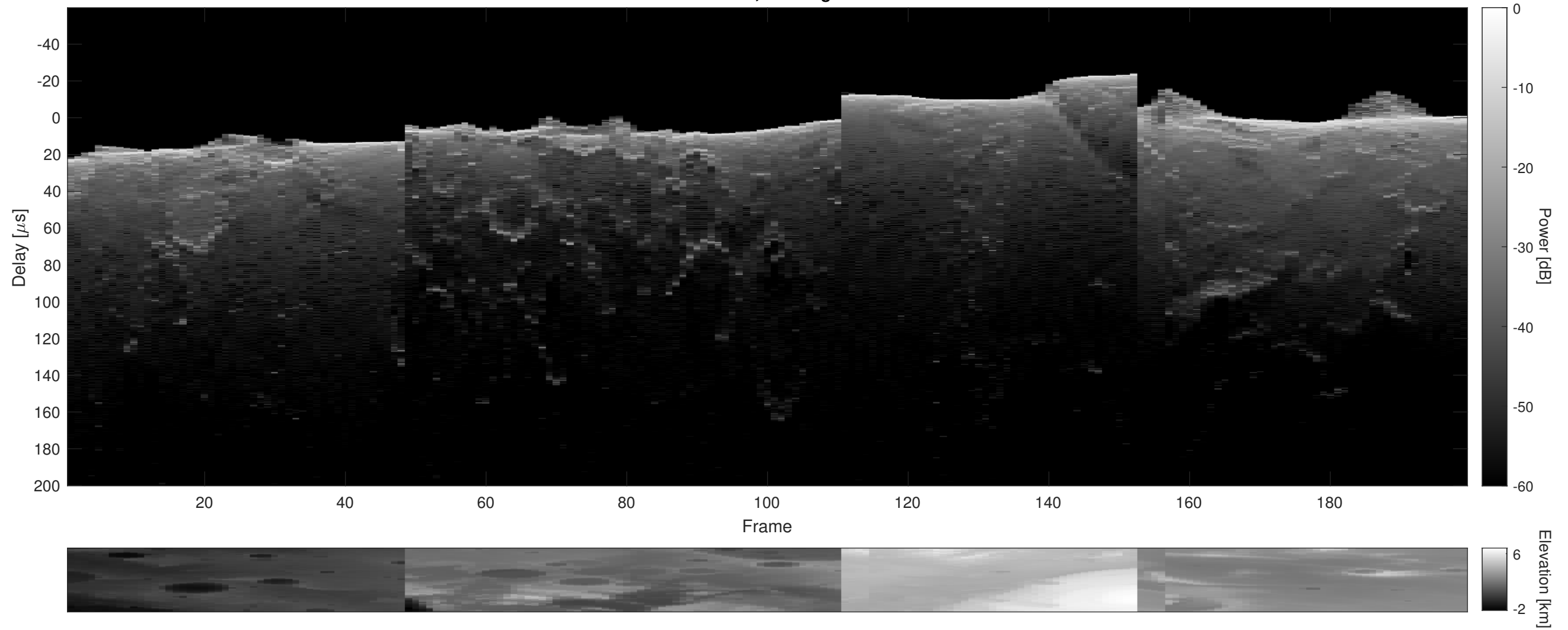
Orbit 2733, Cluttergram
