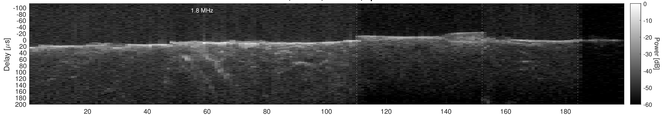
Orbit 2733, Cluttergram
