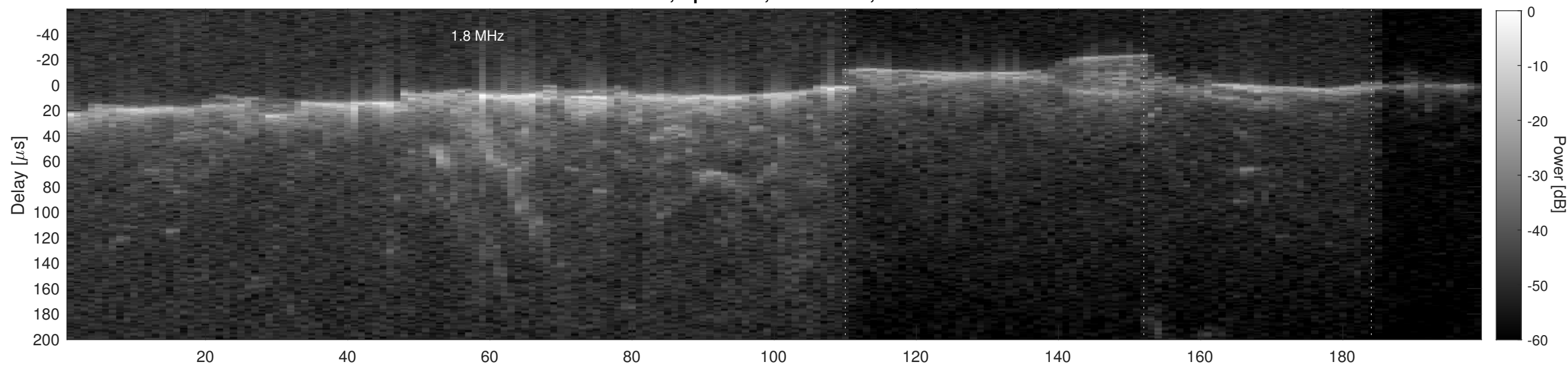
Orbit 2733, Cluttergram
