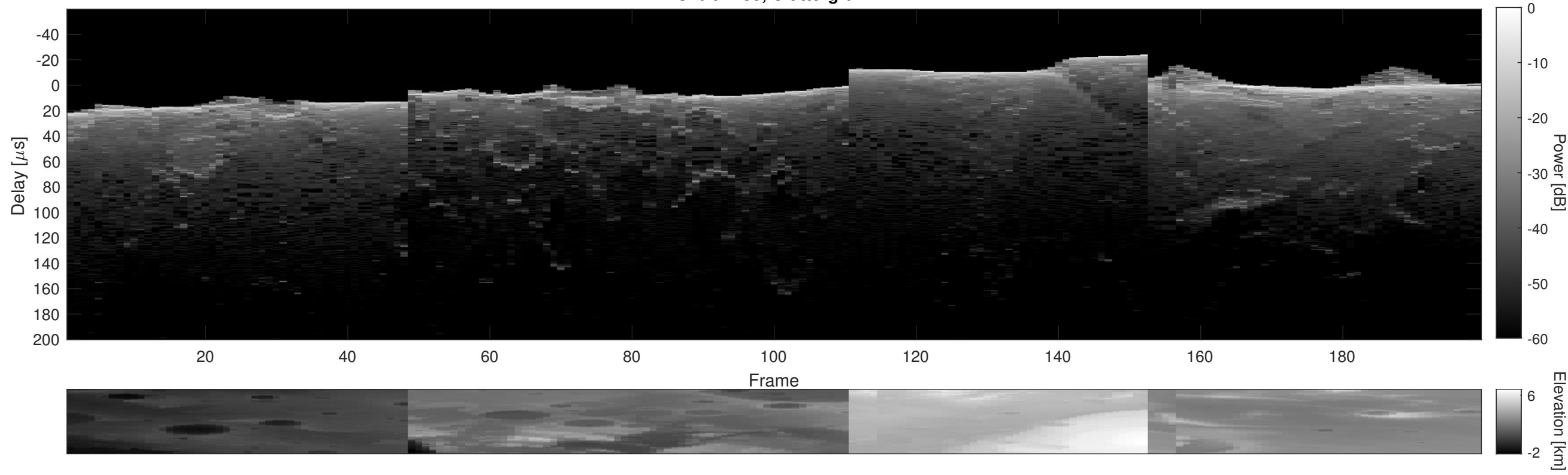
Orbit 2733, Cluttergram
