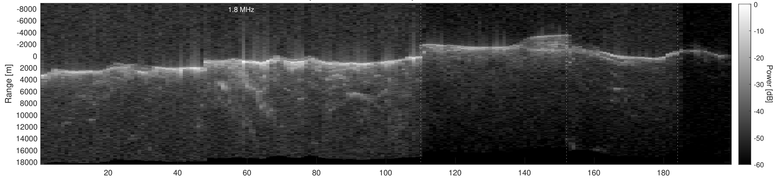
Orbit 2733, Depth-Corrected Cluttergram
