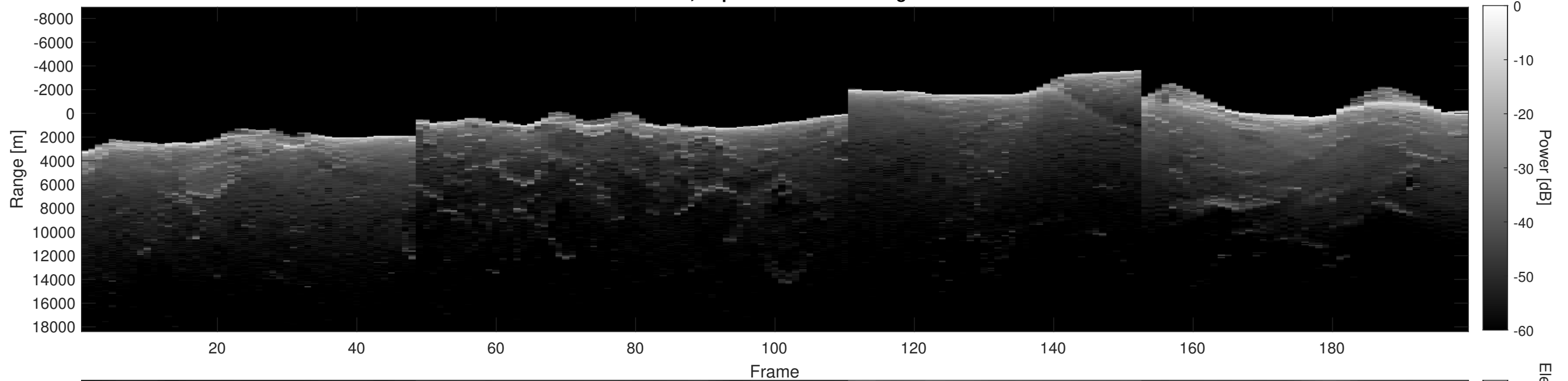
Orbit 2733, Depth-Corrected Cluttergram
