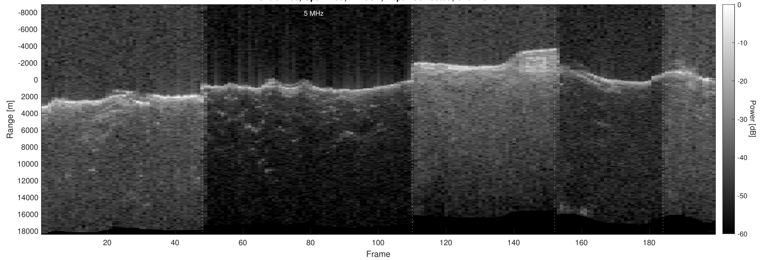
Orbit 2733, Optimized, Window, Depth-Corrected, Channel 2
