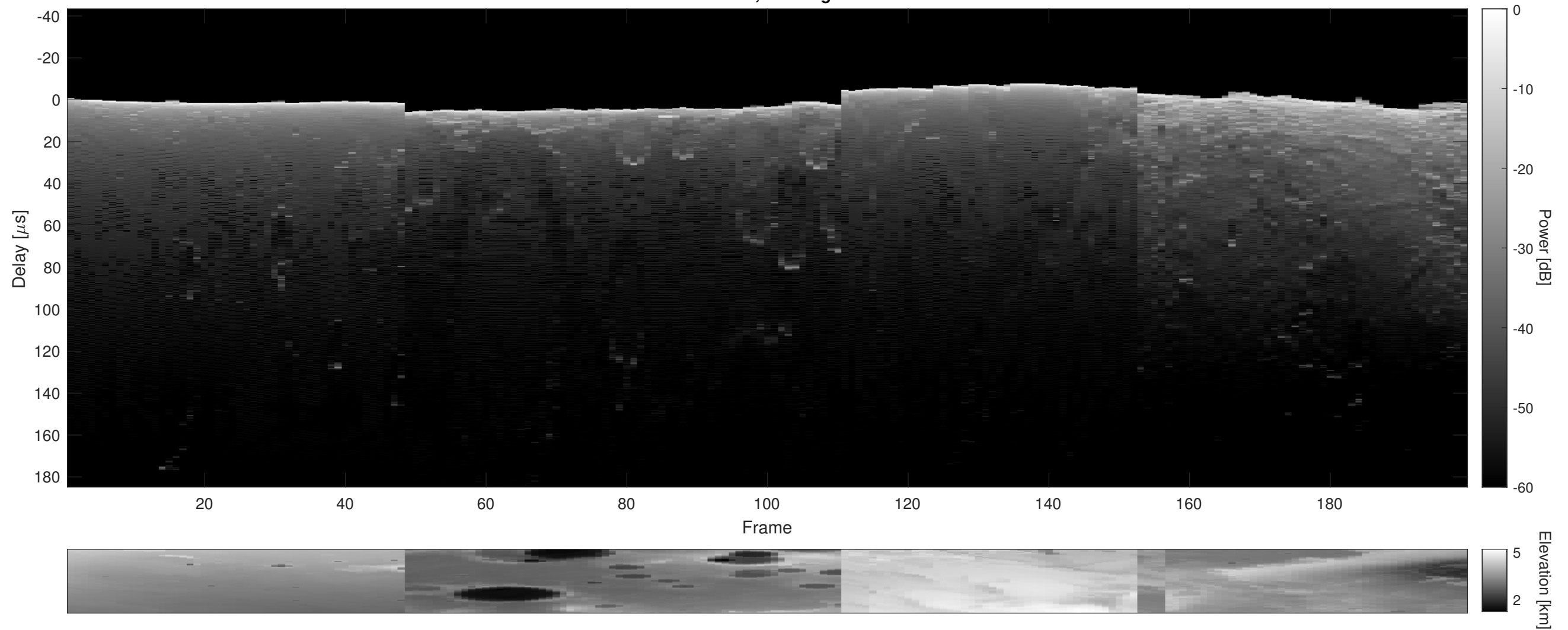
Orbit 2734, Cluttergram
