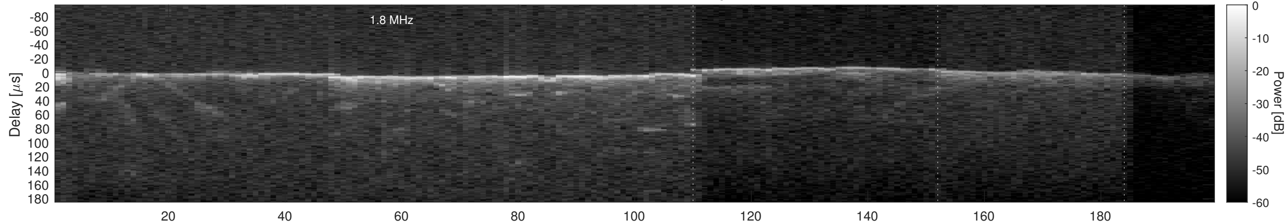
Orbit 2734, Cluttergram
