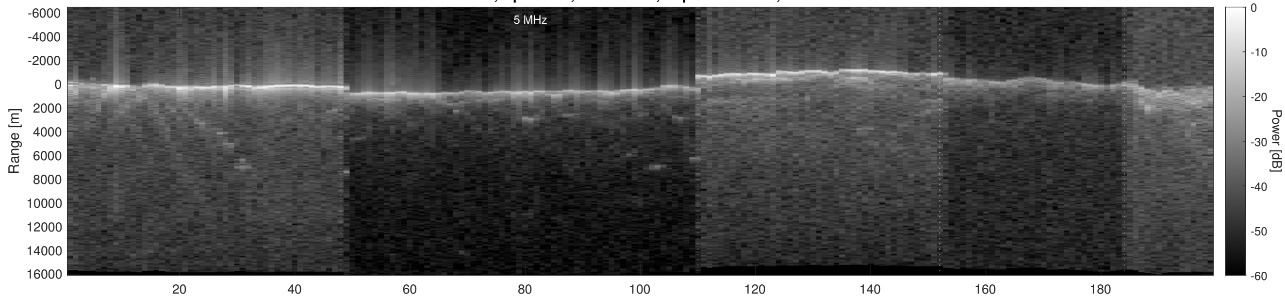
Orbit 2734, Optimized, No Window, Depth-Corrected, Channel 2
