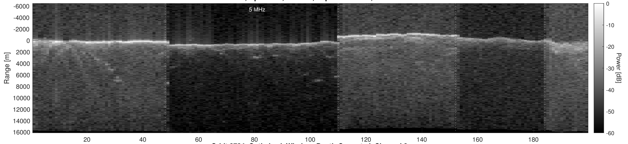
Orbit 2734, Optimized, Window, Depth-Corrected, Channel 2
