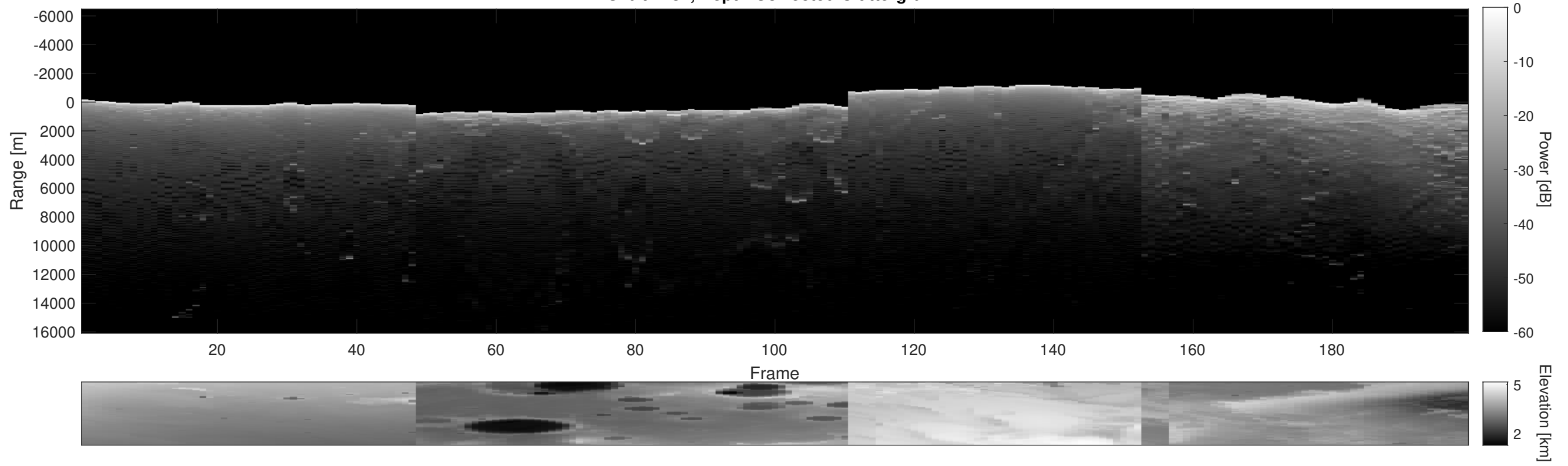
Orbit 2734, Depth-Corrected Cluttergram
