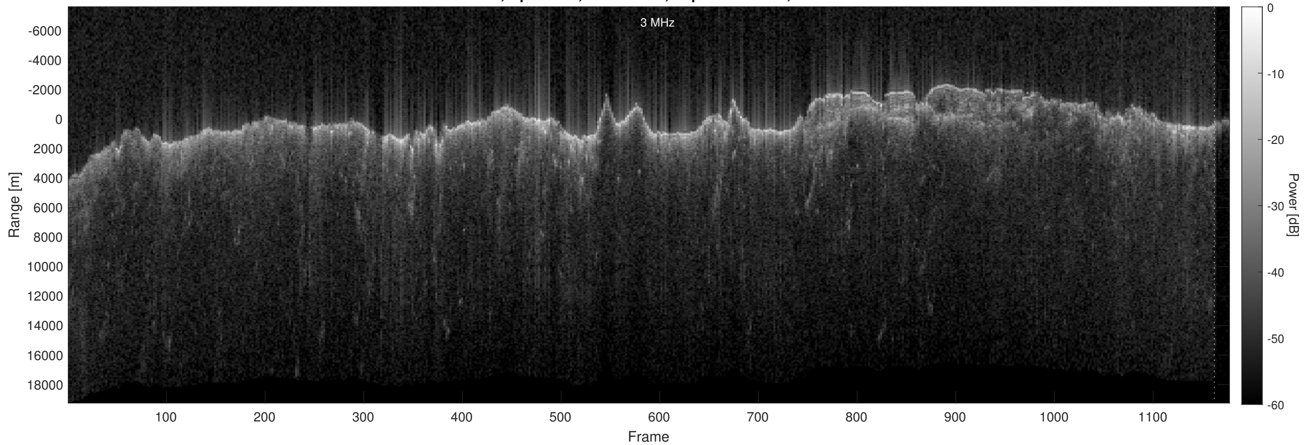
Orbit 2735, Optimized, No Window, Depth-Corrected, Channel 2
