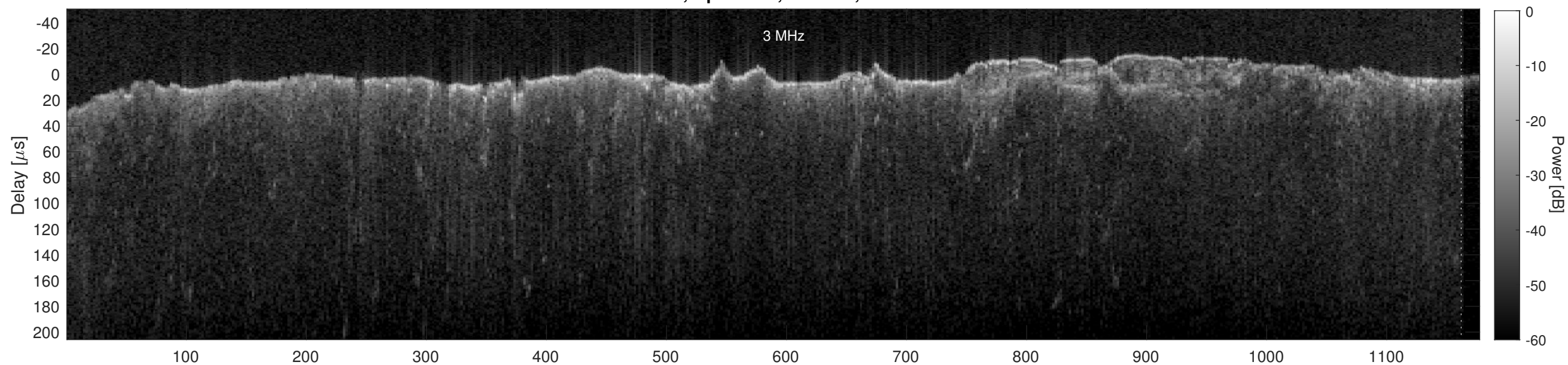
Orbit 2735, Cluttergram
