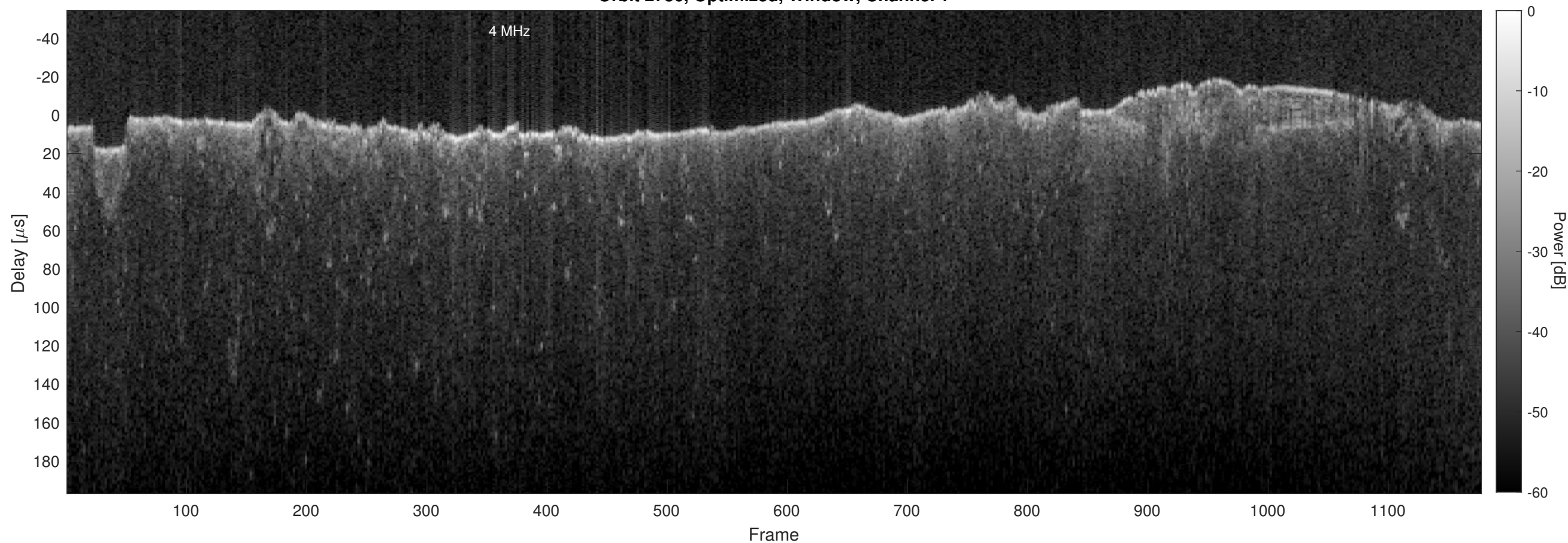
Orbit 2736, Optimized, Window, Channel 2
