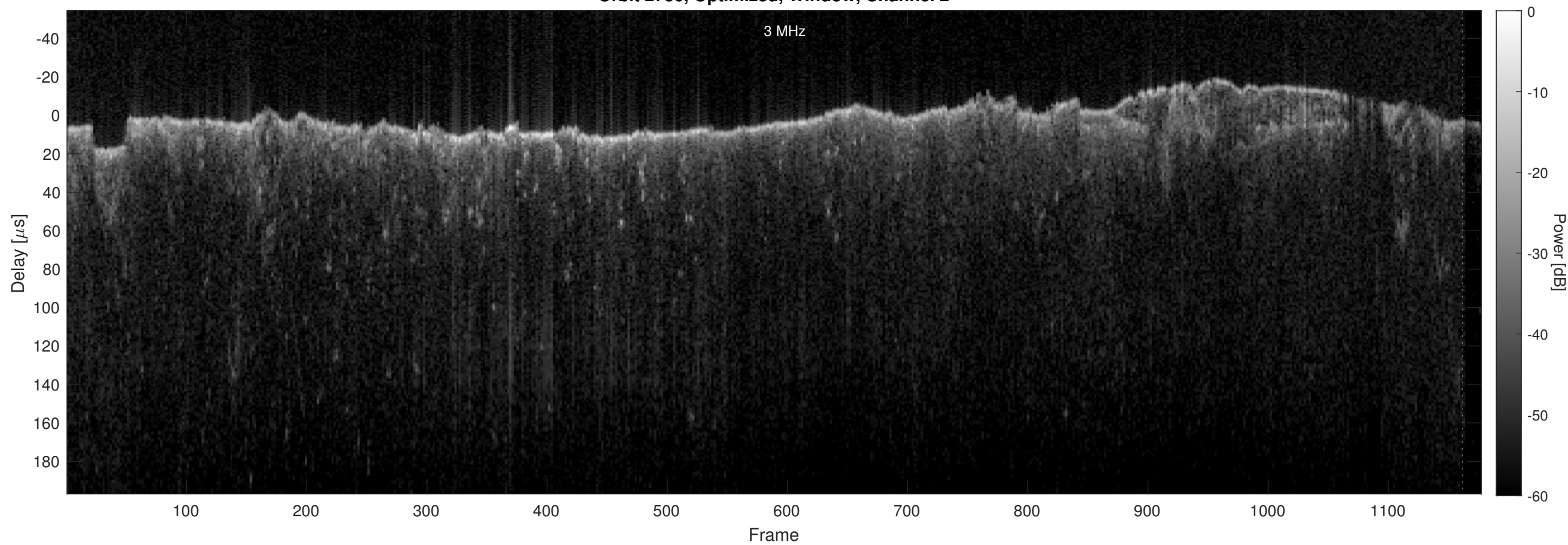
Orbit 2736, Optimized, Window, Channel 2
