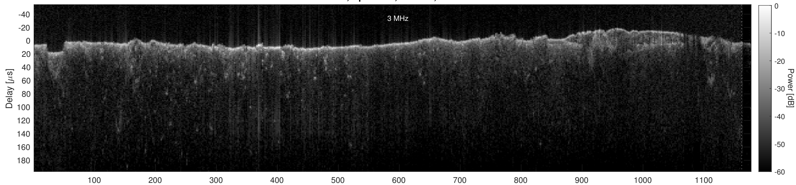
Orbit 2736, Cluttergram
