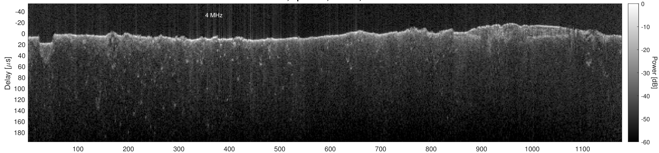
Orbit 2736, Optimized, Window, Channel 2
