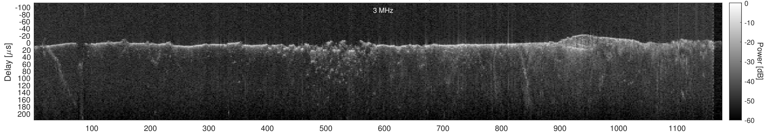
Orbit 2737, Cluttergram
