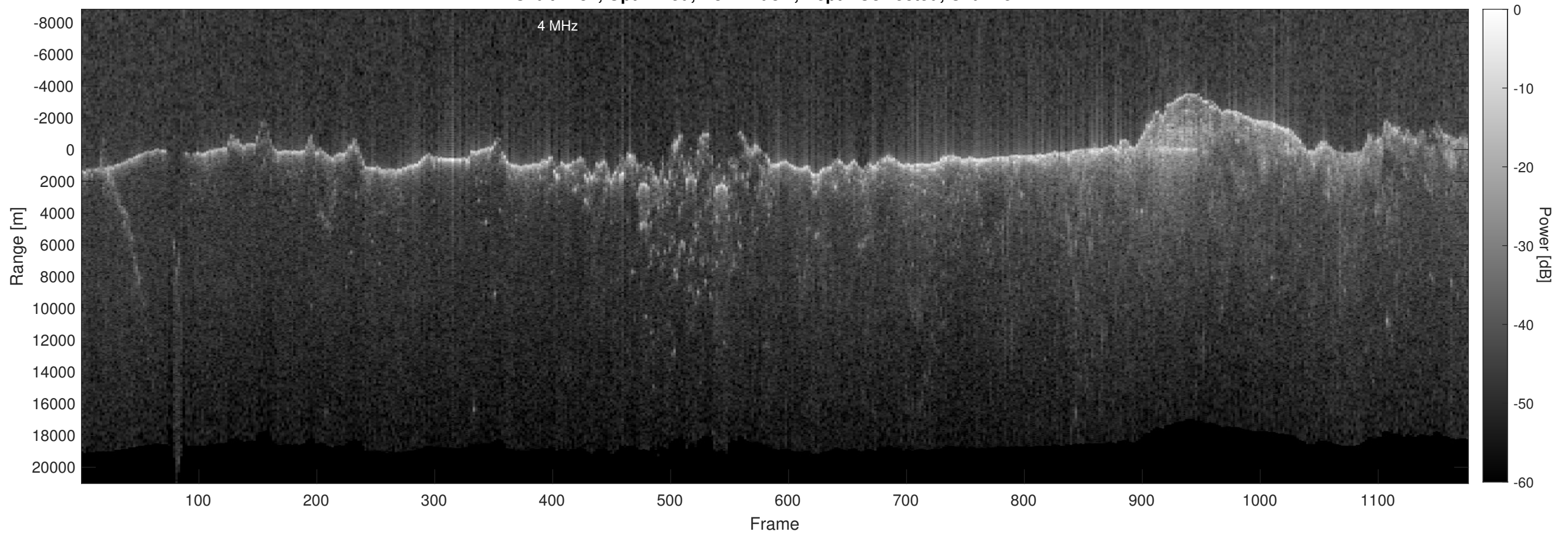
Orbit 2737, Optimized, No Window, Depth-Corrected, Channel 2
