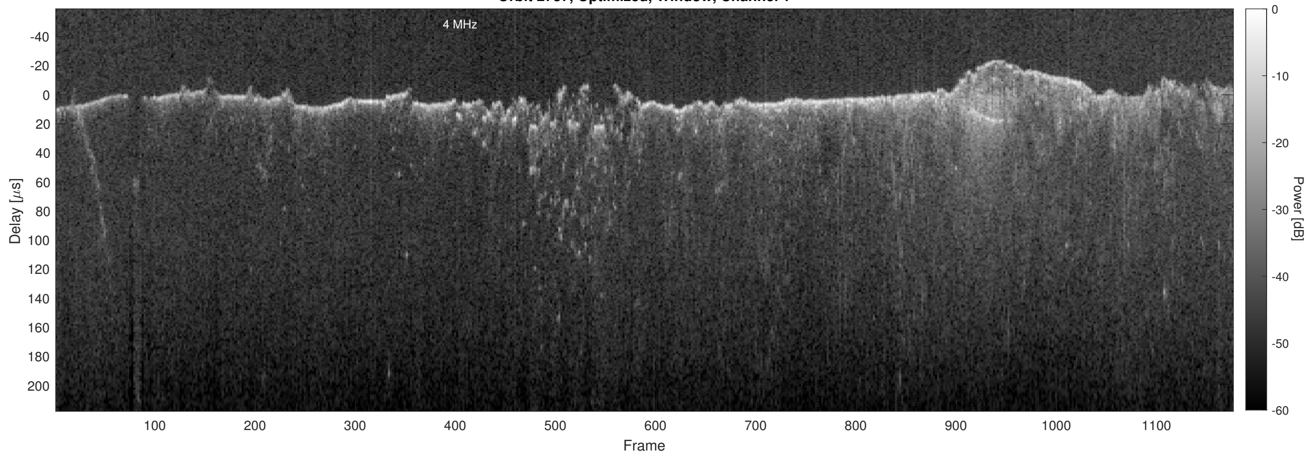
Orbit 2737, Optimized, Window, Channel 2
