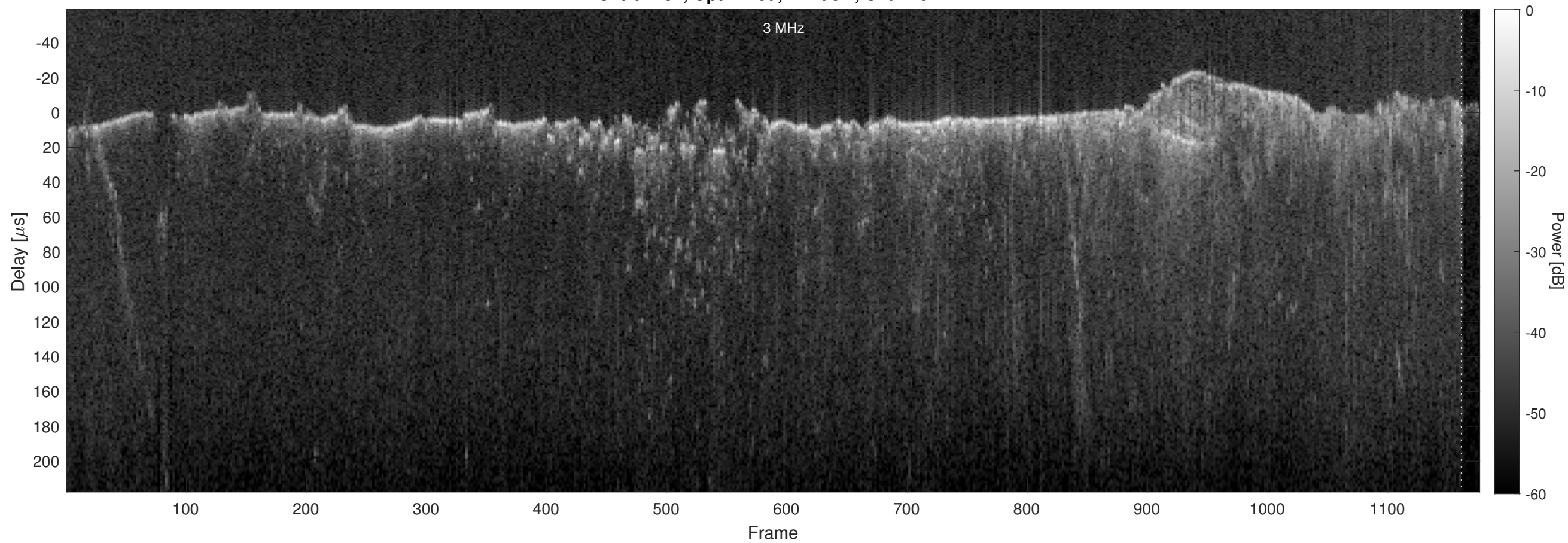
Orbit 2737, Optimized, Window, Channel 2
