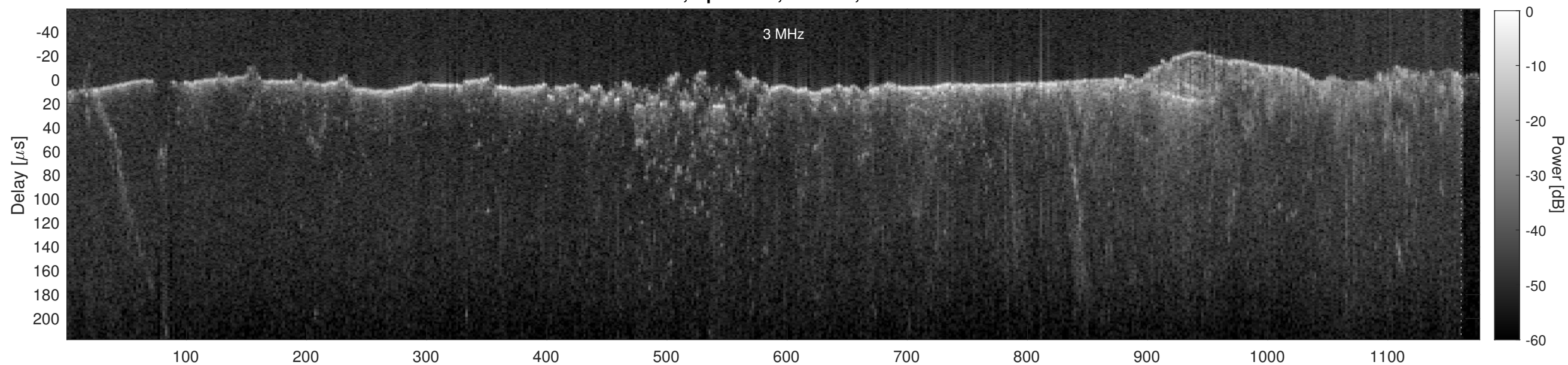
Orbit 2737, Cluttergram
