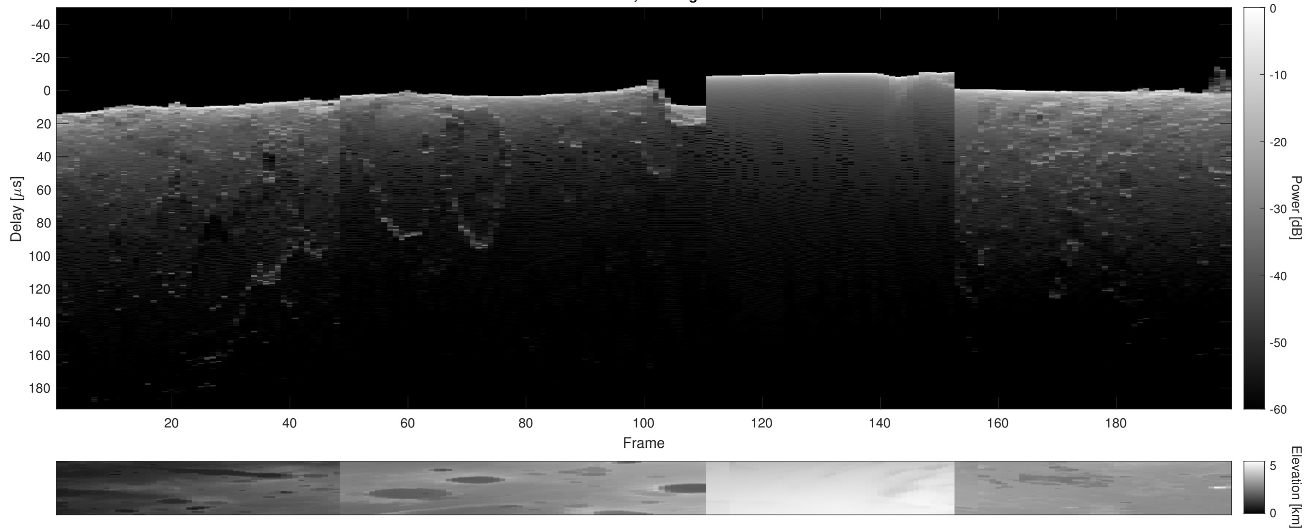
Orbit 2738, Cluttergram
