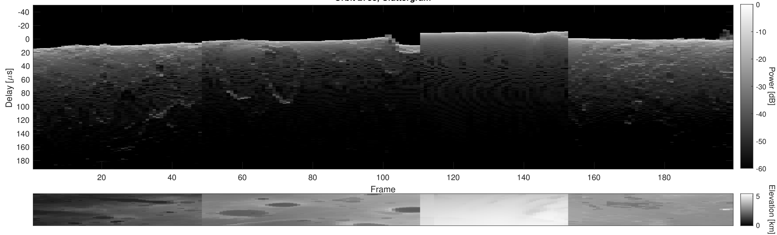
Orbit 2738, Cluttergram
