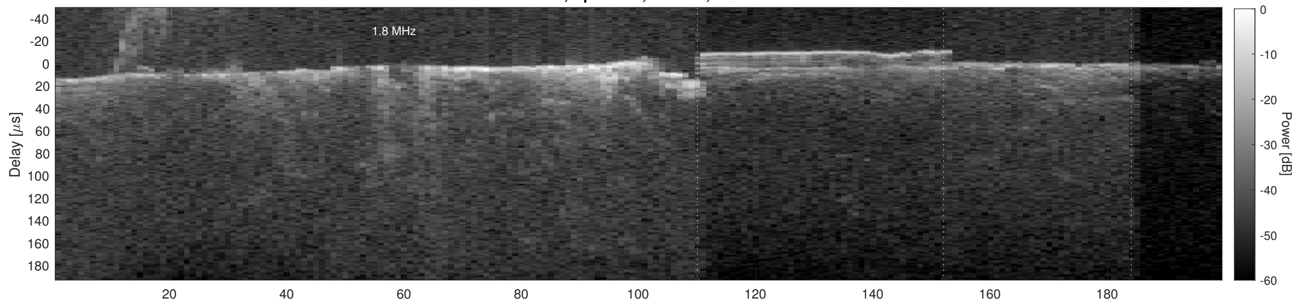
Orbit 2738, Cluttergram
