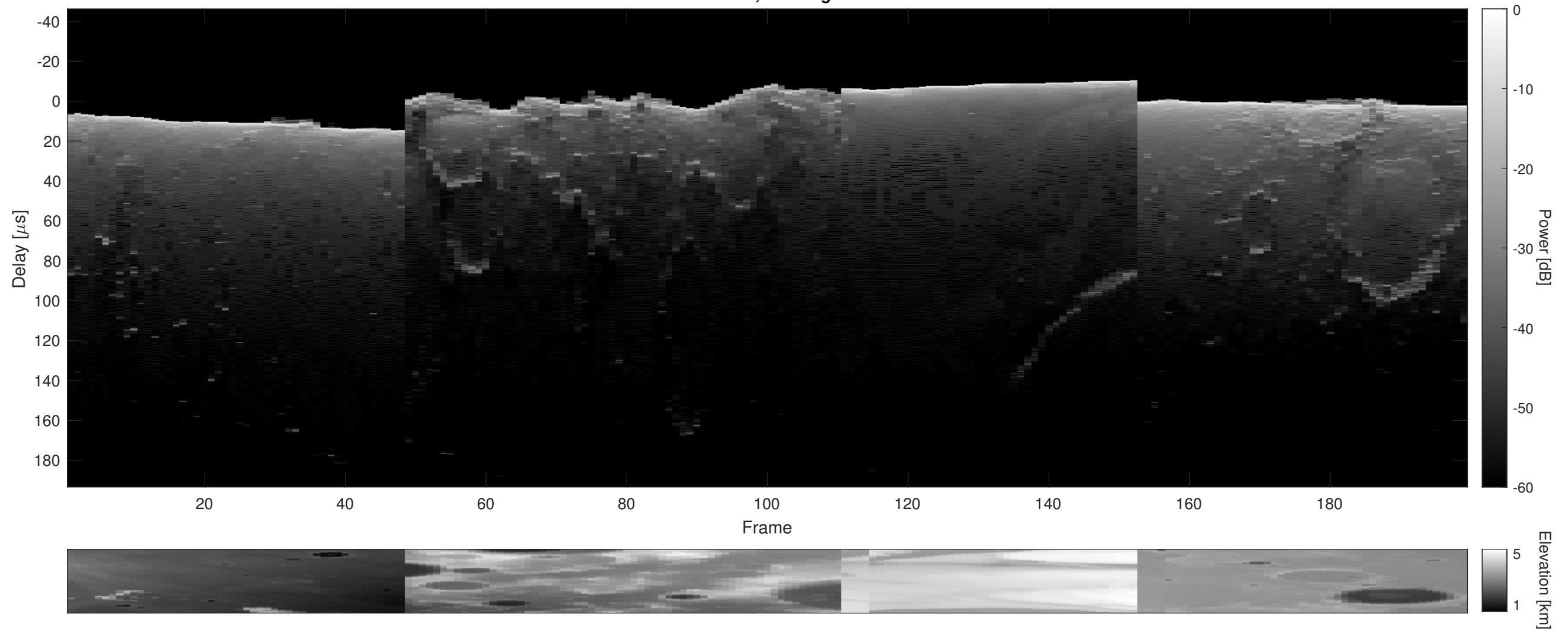
Orbit 2739, Cluttergram
