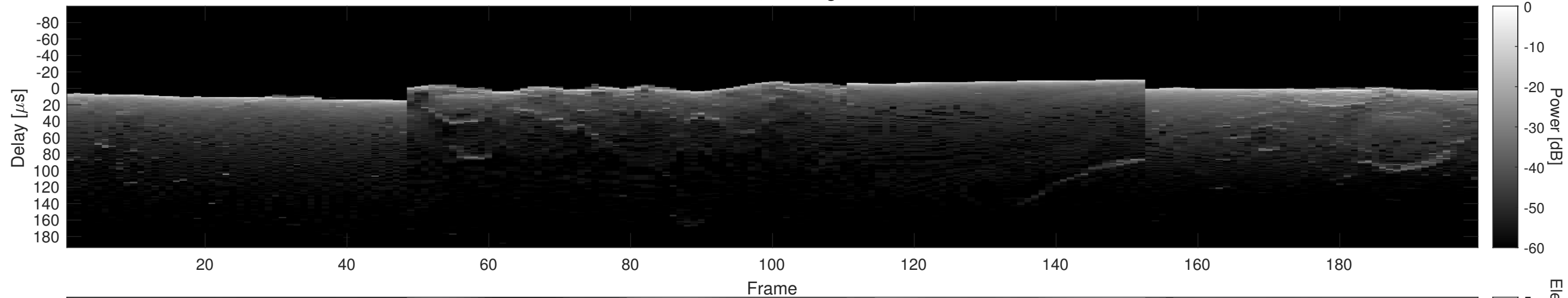
Orbit 2739, Cluttergram
