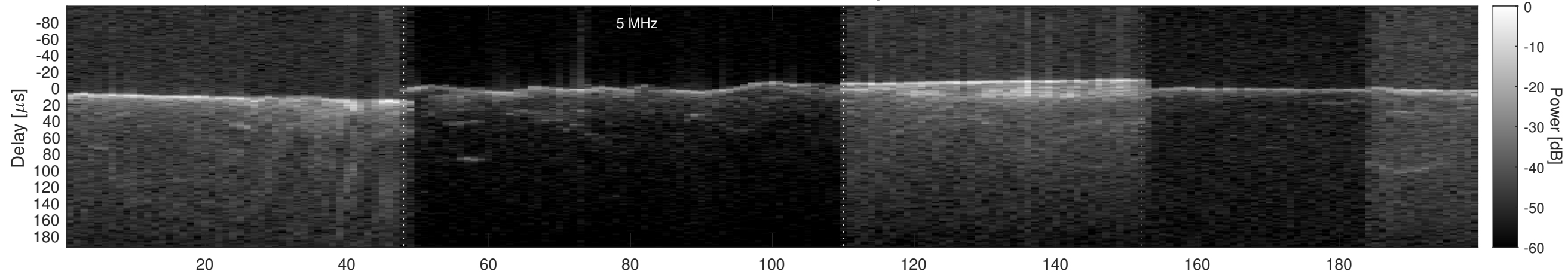
Orbit 2739, Cluttergram
