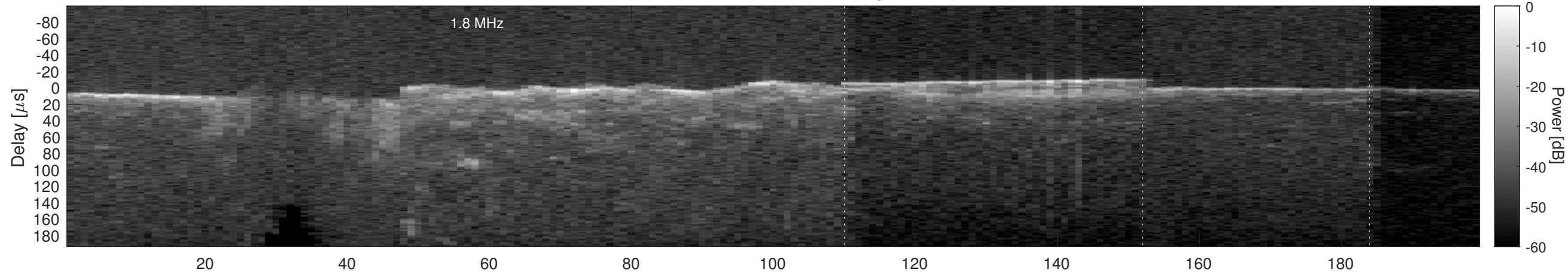
Orbit 2739, Cluttergram
