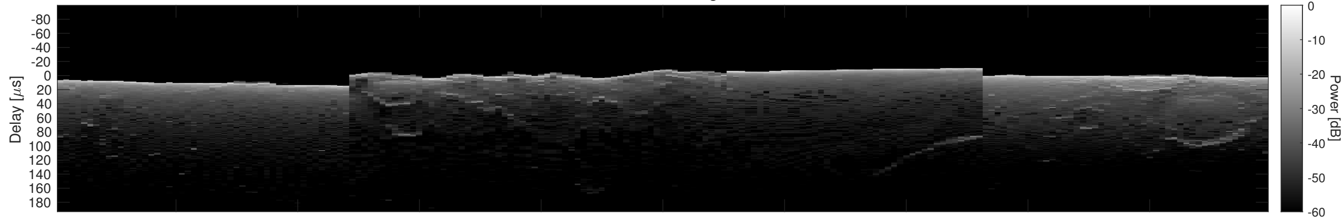
Orbit 2739, Cluttergram
