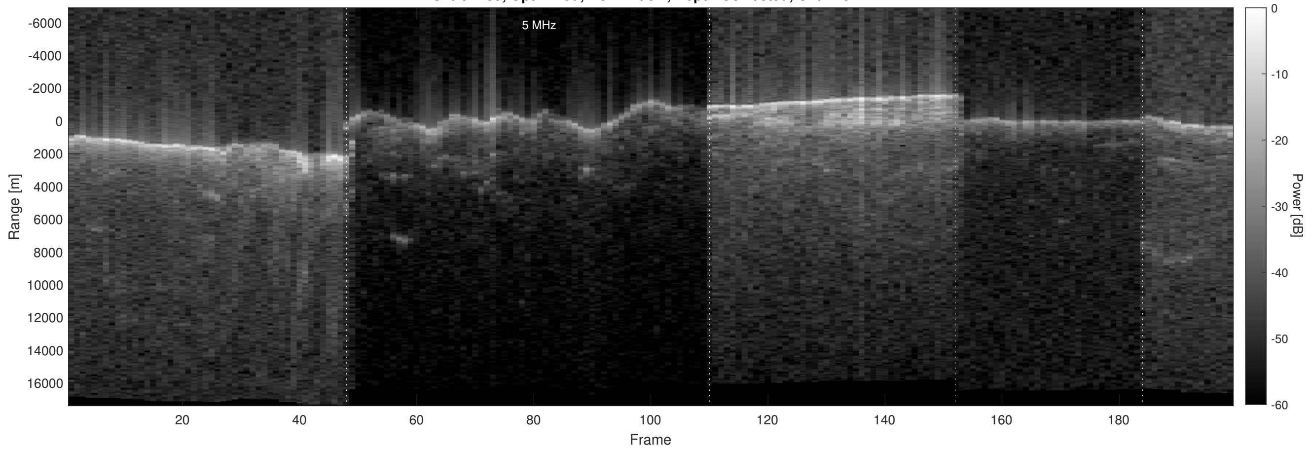
Orbit 2739, Optimized, No Window, Depth-Corrected, Channel 2
