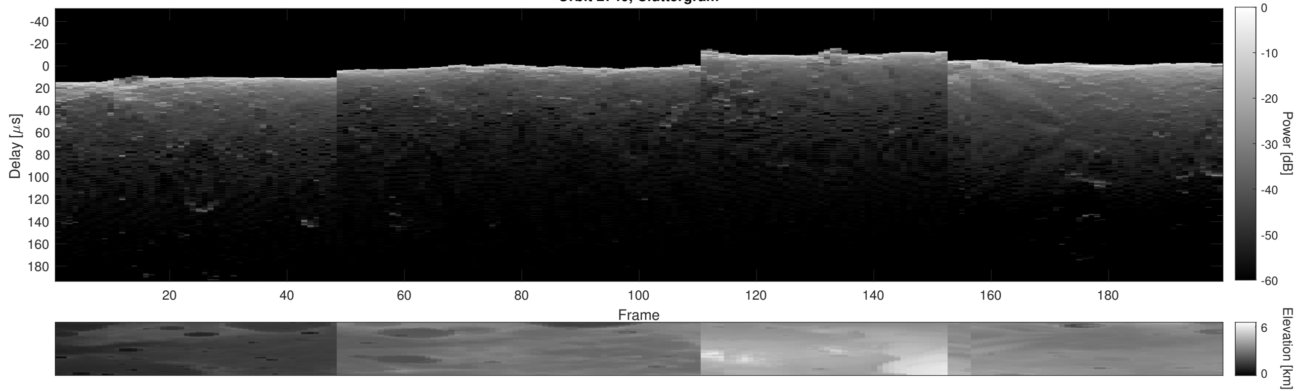
Orbit 2740, Cluttergram
