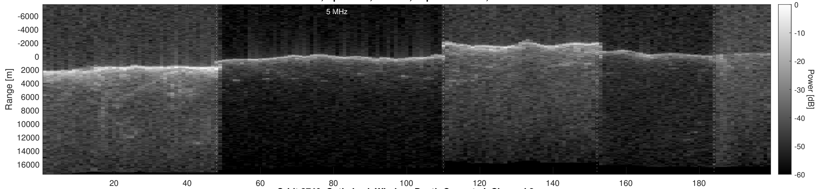
Orbit 2740, Optimized, Window, Depth-Corrected, Channel 2
