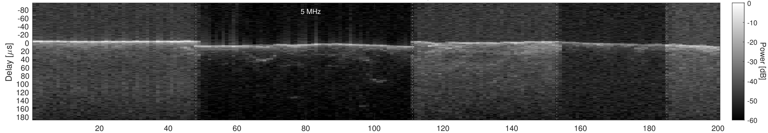
Orbit 2741, Cluttergram
