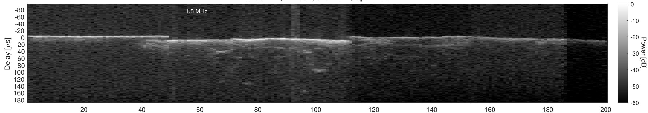
Orbit 2741, Cluttergram
