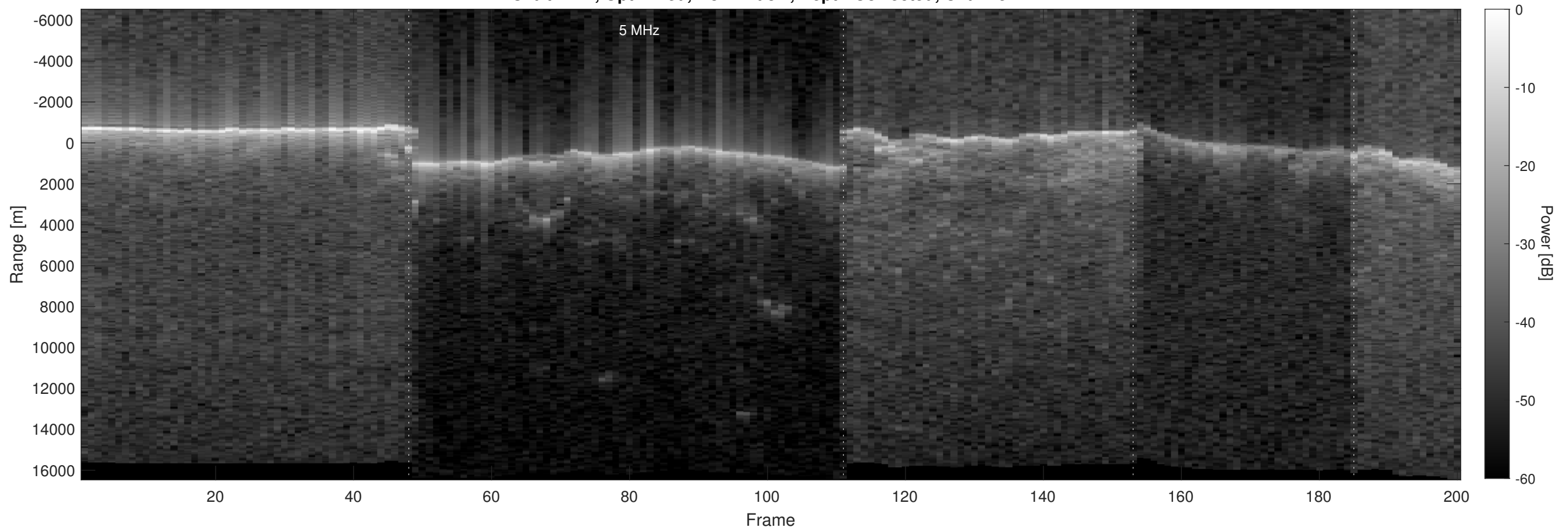
Orbit 2741, Optimized, No Window, Depth-Corrected, Channel 2
