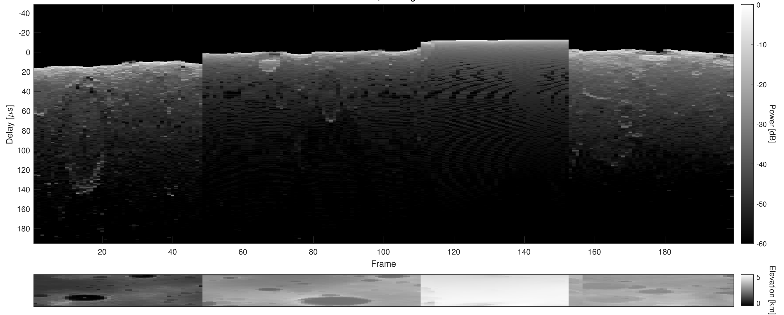
Orbit 2742, Cluttergram
