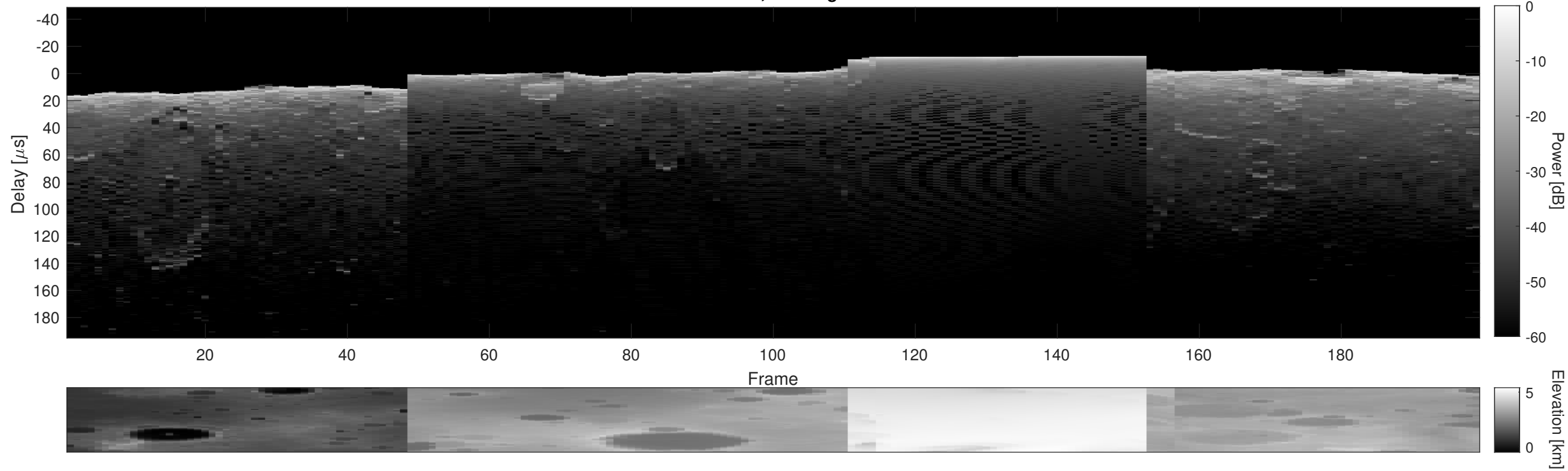
Orbit 2742, Cluttergram
