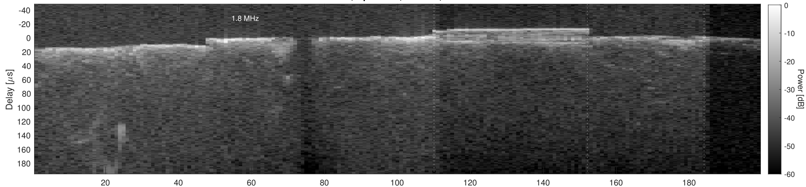
Orbit 2742, Cluttergram
