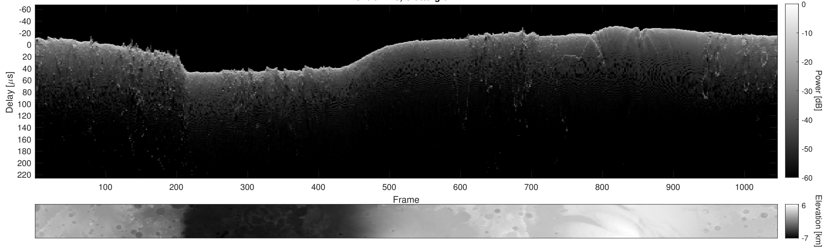
Orbit 2743, Cluttergram
