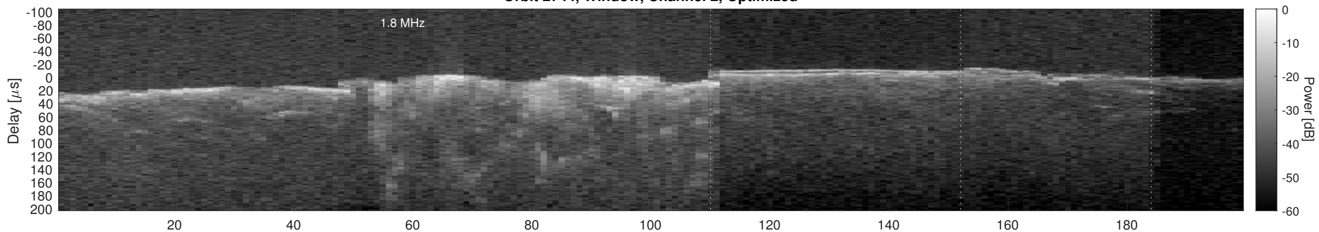
Orbit 2744, Cluttergram
