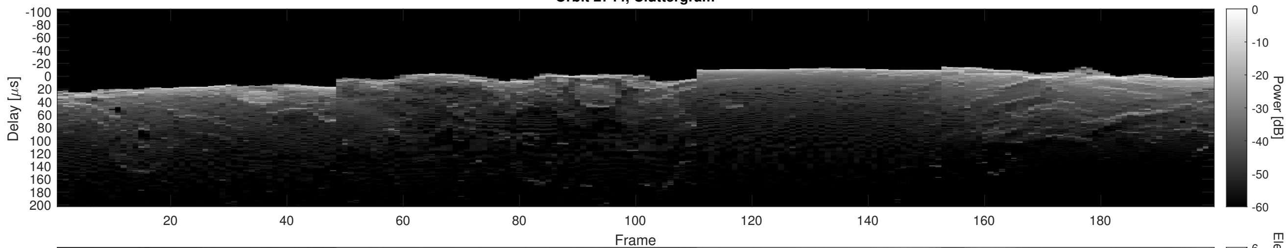
Orbit 2744, Cluttergram
