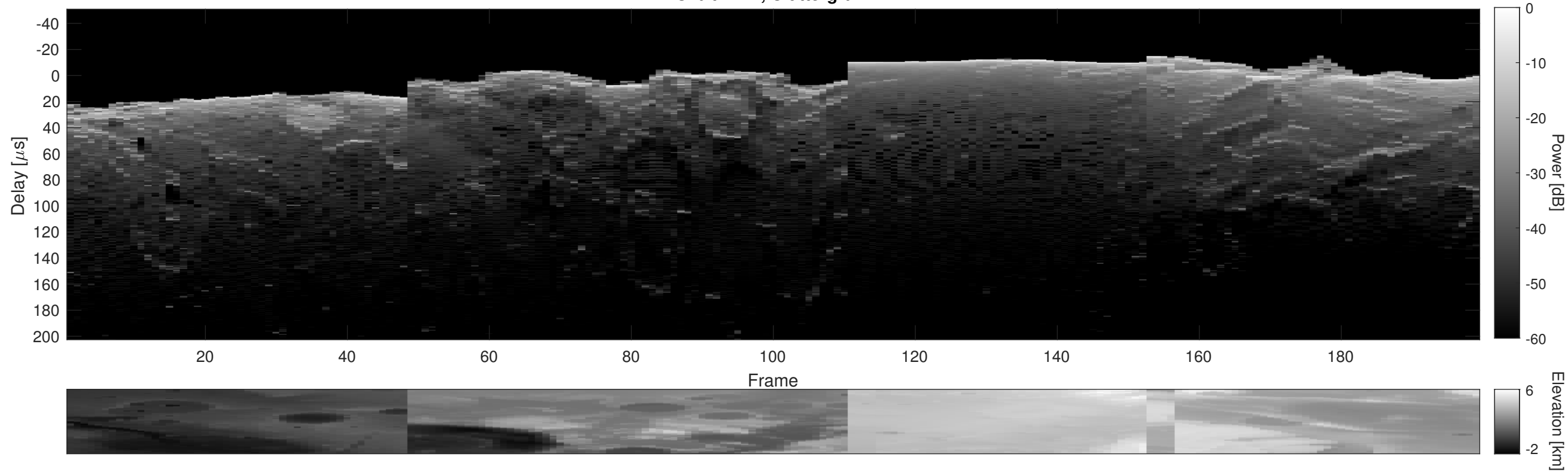
Orbit 2744, Cluttergram
