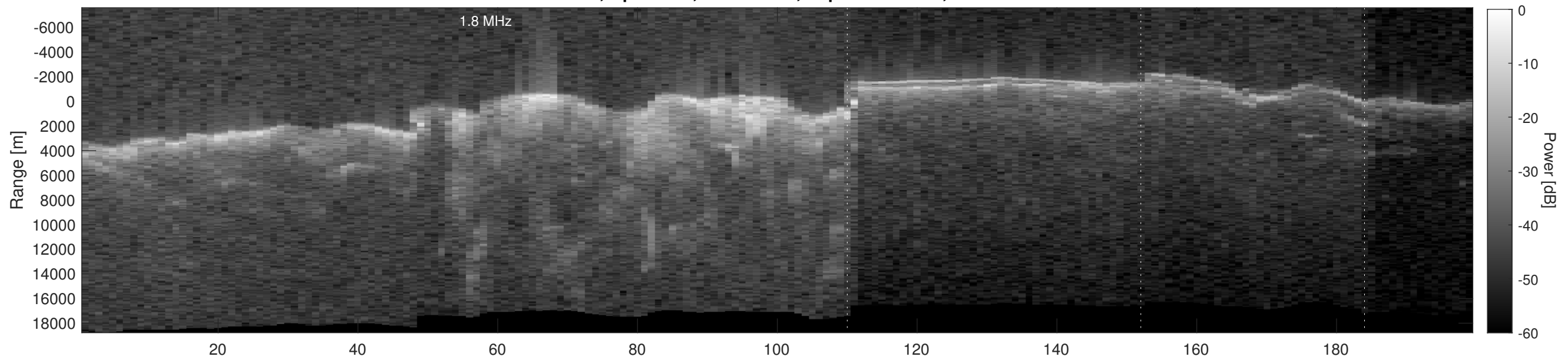
Orbit 2744, Depth-Corrected Cluttergram
