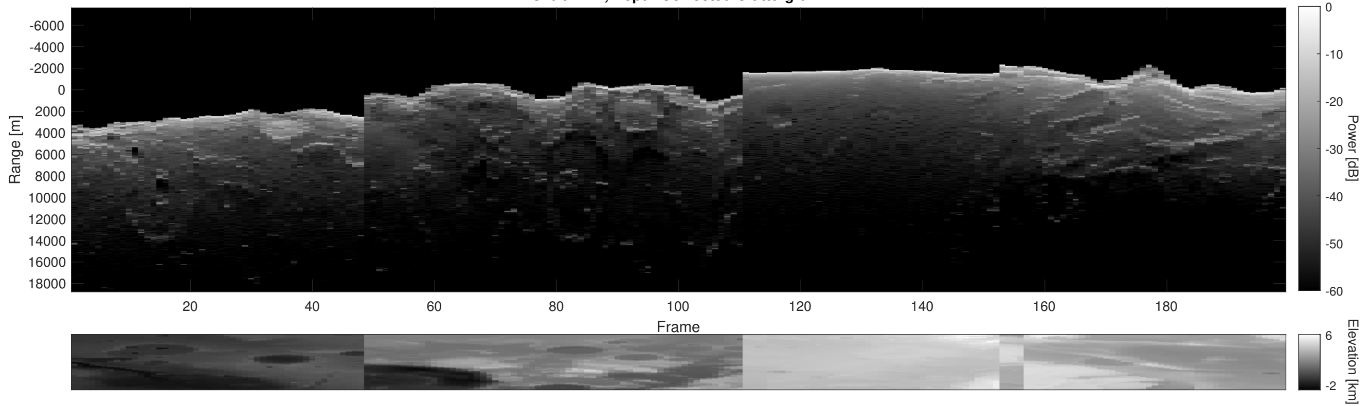
Orbit 2744, Depth-Corrected Cluttergram
