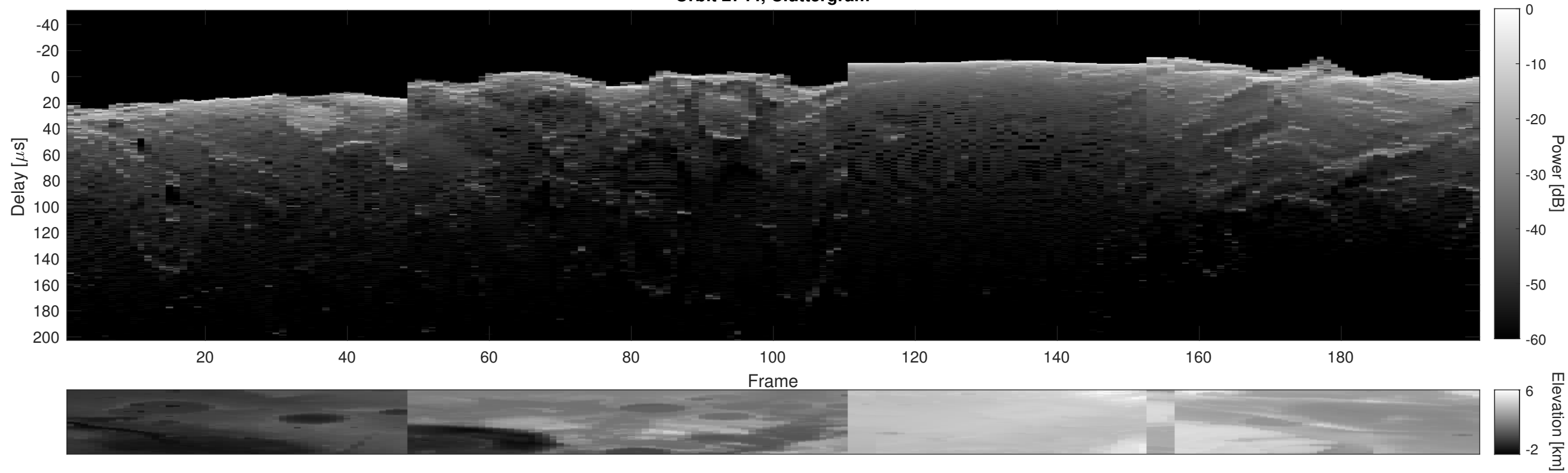
Orbit 2744, Cluttergram
