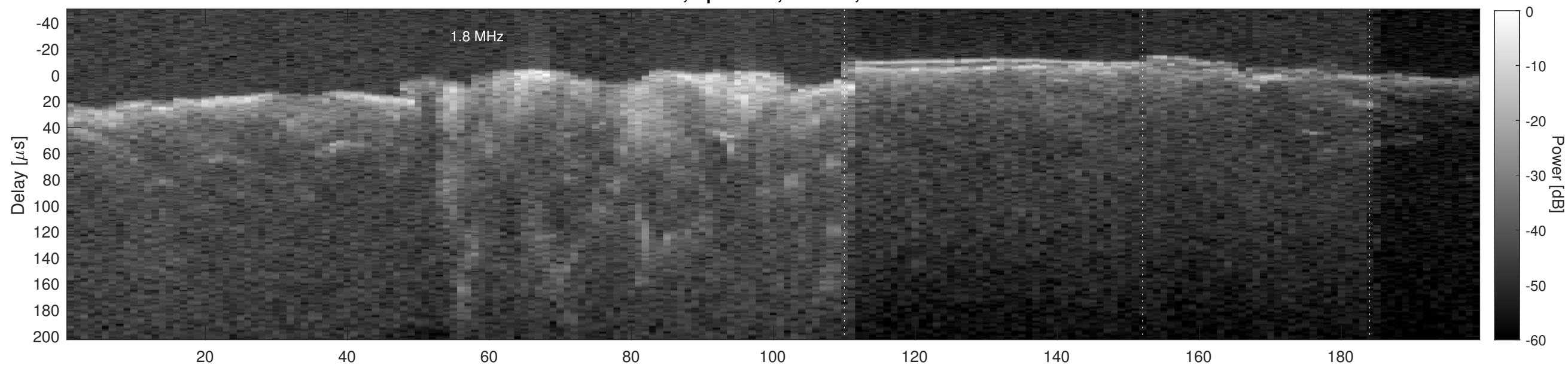
Orbit 2744, Cluttergram
