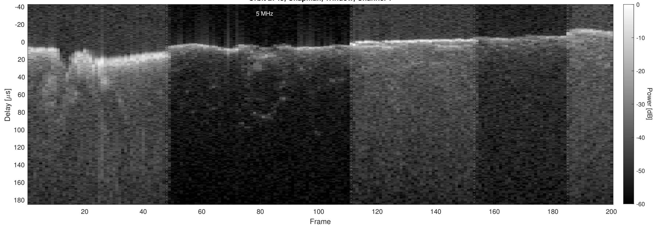
Orbit 2745, Chapman, Window, Channel 2
