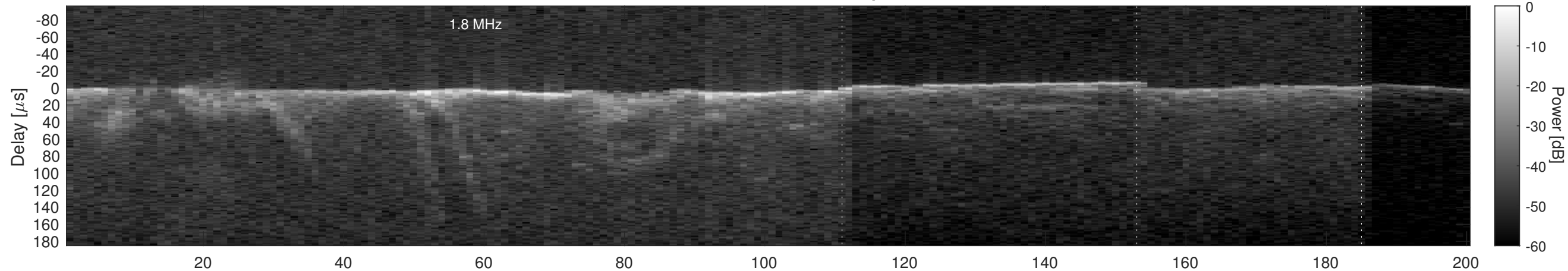
Orbit 2745, Cluttergram
